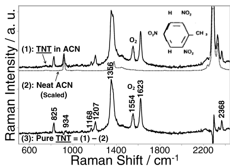
FIG. 4. 229 nm UV Raman spectra of TNT not corrected for self-absorption. (1) 2 mg/mL TNT in ACN, (2) pure ACN, (3) pure TNT spectrum, with ACN contribution numerically removed. The 1554 \text{cm}^{-1} band derives from oxygen in the air.
